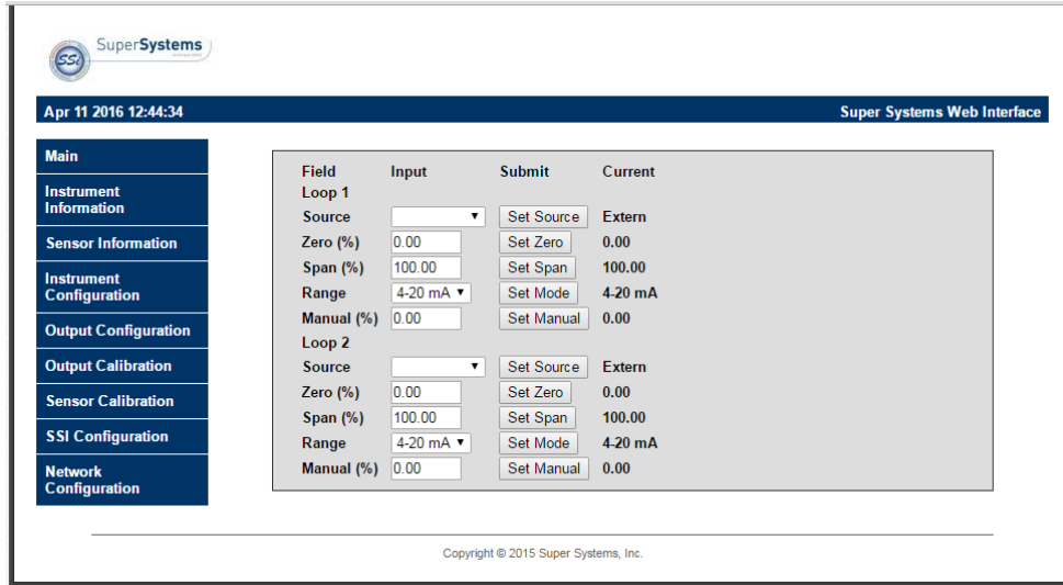
Figure 7 - Output Configuration Page
