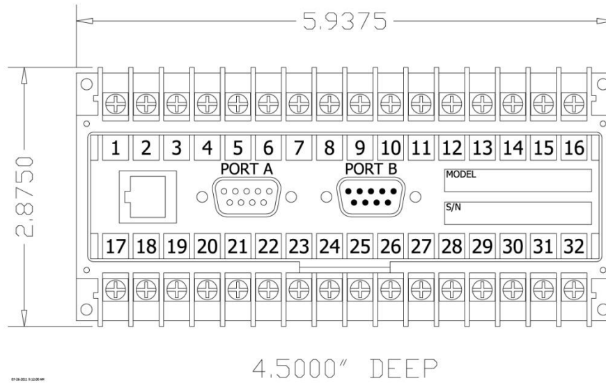
Series 9205 Controller Dimensions
